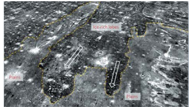
Thermal image showing ice-rich lobes, dark and outlined in yellow, believed to be remnants of tsunami waves that became slurry ice-rich flows that spread in extremely cold climate conditions. White arrows indicate flow going upslope. The lobe is about 250 km in length. Credit: NASA/JPL.
