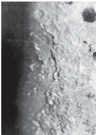
The best of Bill Hartmann's discovery images, showing the rings of the giant Orientale impact basin, as published in 1962.
