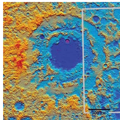
A 2010 topographic map, shows the entire Orientale basin system of concentric and radial fractures. The white box shows the part of the ring system that appears at left. The outer ring is about 1200 km across, 1/3 the size of the moon itself. Credit: Lunar Reconnaissance Orbiter Laser Altimeter Map
