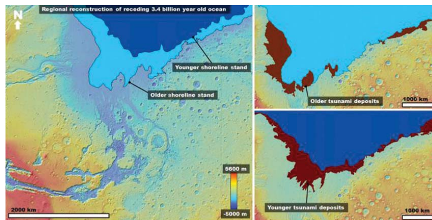
At left, a color-coded digital elevation model of the study area showing the two proposed shoreline levels of an early Mars ocean that existed circa 3.4 billion years ago. At right, the areas covered by the documented tsunami events extending from these shorelines.
