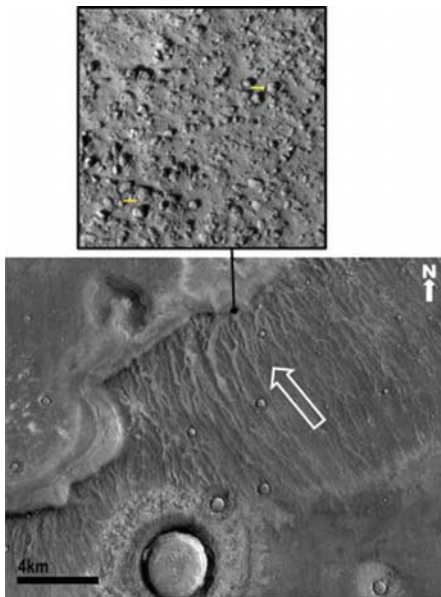
View of boulder-rich surface (yellow bars are 10 m) deposited by the older tsunami and then eroded by channels produced as the tsunami water returned to the ocean elevation level.
